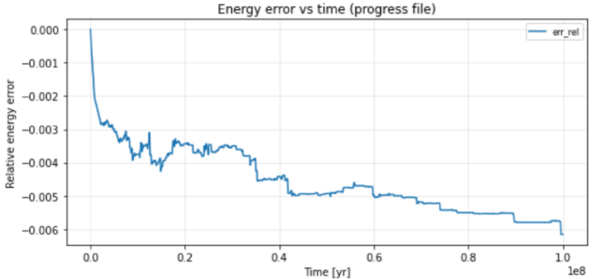
Figure 7. from Samuele Crespi et al 2026 Astron. J. 172 doi:10.3847/1538-3881/ae8ae7 https://dx.doi.org/10.3847/1538-3881/ae8ae7 © 2026. The Author(s). Published by the American Astronomical Society.
