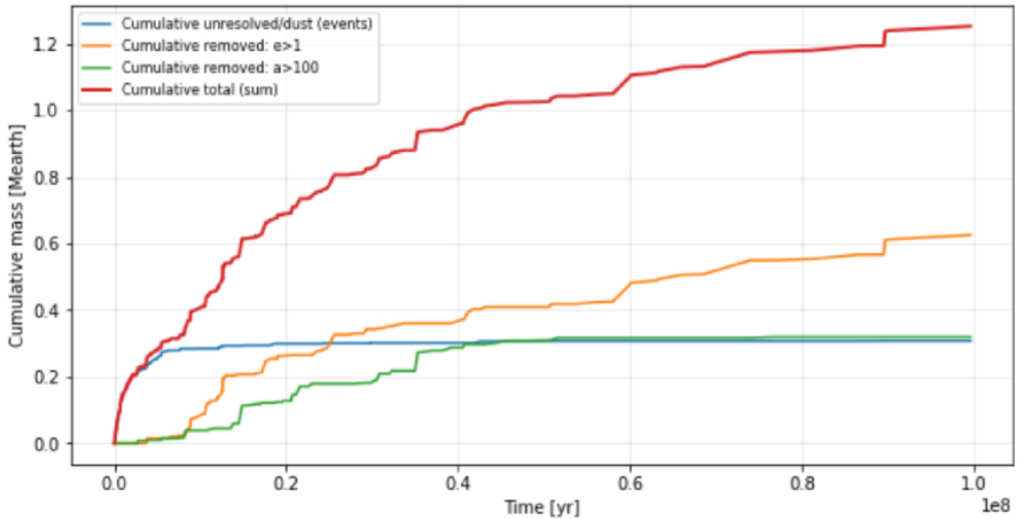
Figure 5. from Samuele Crespi et al 2026 Astron. J. 172 doi:10.3847/1538-3881/ae8ae7 https://dx.doi.org/10.3847/1538-3881/ae8ae7 © 2026. The Author(s). Published by the American Astronomical Society.
