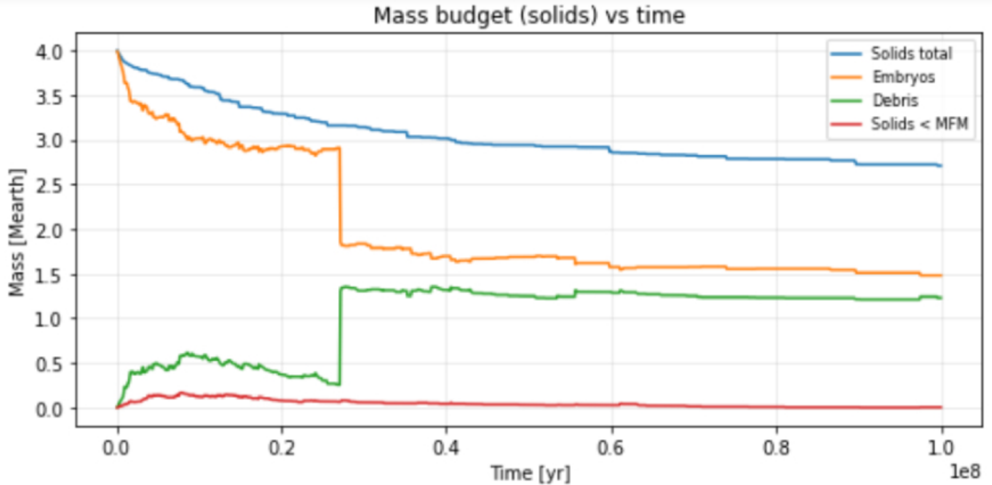
Figure 4. from Samuele Crespi et al 2026 Astron. J. 172 doi:10.3847/1538-3881/ae8ae7 https://dx.doi.org/10.3847/1538-3881/ae8ae7 © 2026. The Author(s). Published by the American Astronomical Society.
