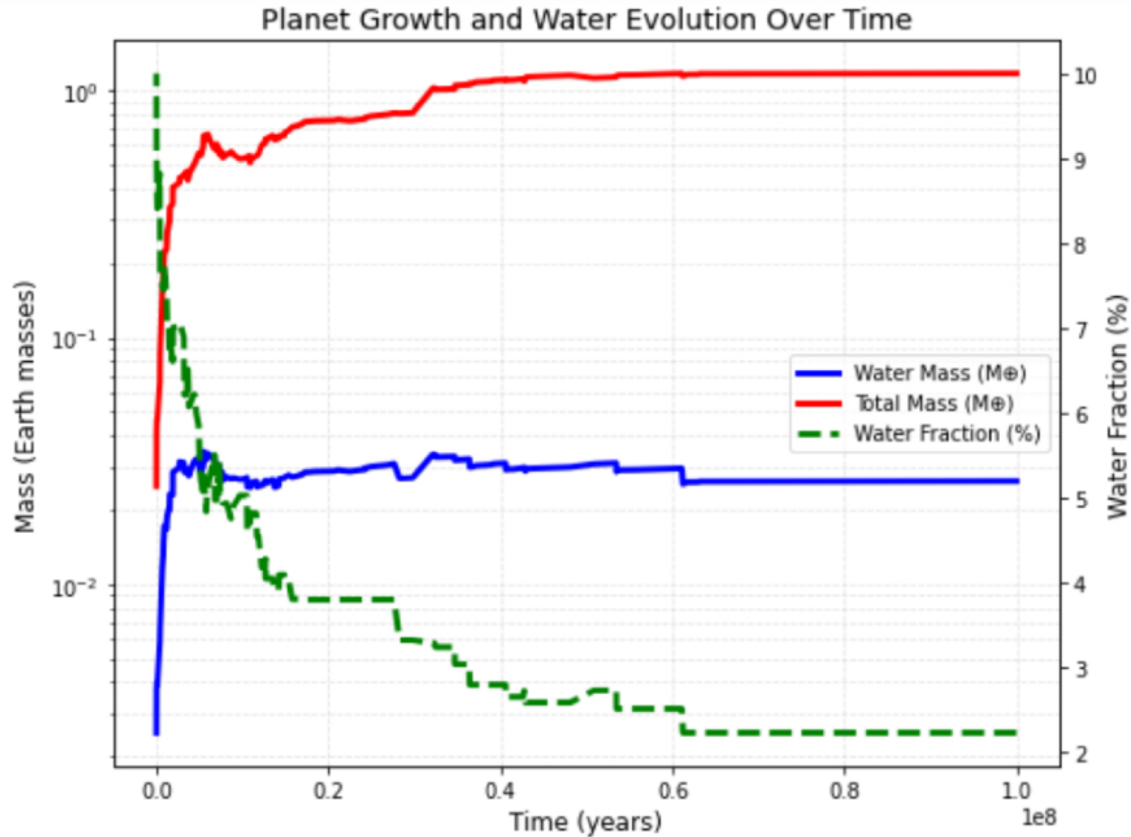
Figure 3. from Samuele Crespi et al 2026 Astron. J. 172 doi:10.3847/1538-3881/ae8ae7 https://dx.doi.org/10.3847/1538-3881/ae8ae7 © 2026. The Author(s). Published by the American Astronomical Society.
