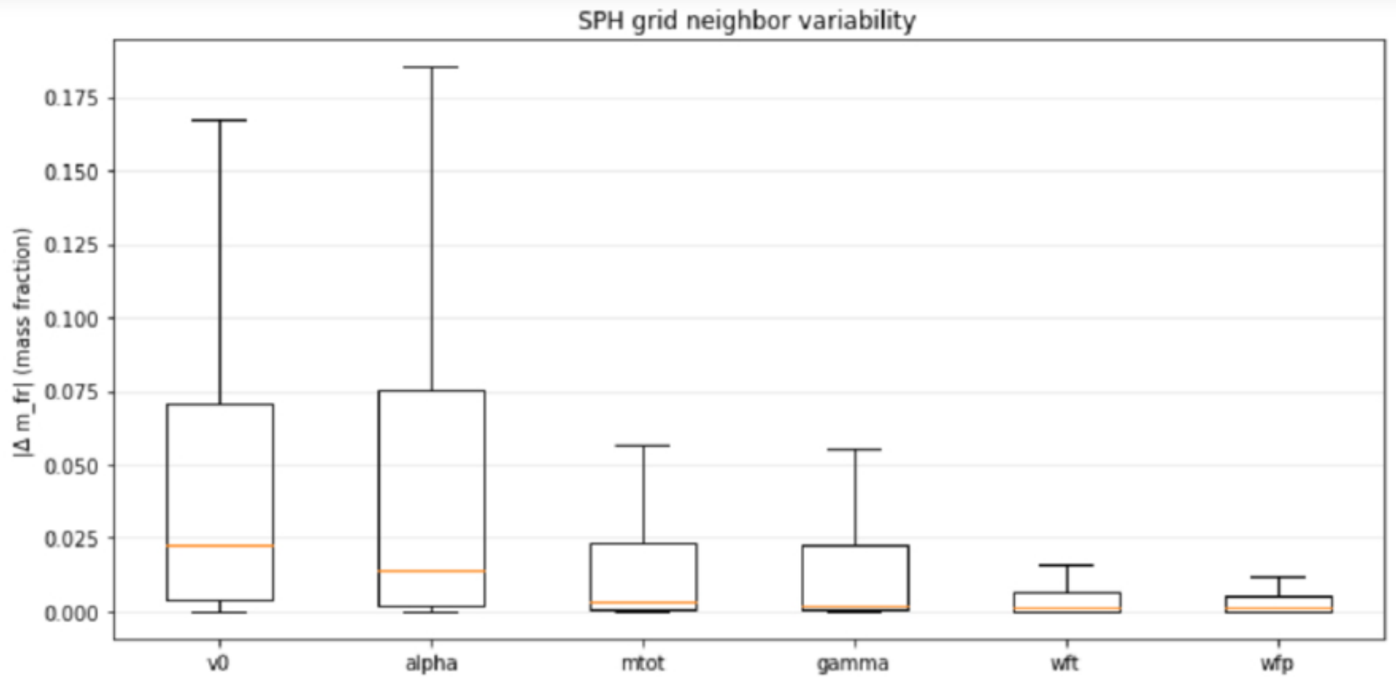
Figure 10. from Samuele Crespi et al 2026 Astron. J. 172 doi:10.3847/1538-3881/ae8ae7 https://dx.doi.org/10.3847/1538-3881/ae8ae7 © 2026. The Author(s). Published by the American Astronomical Society.
