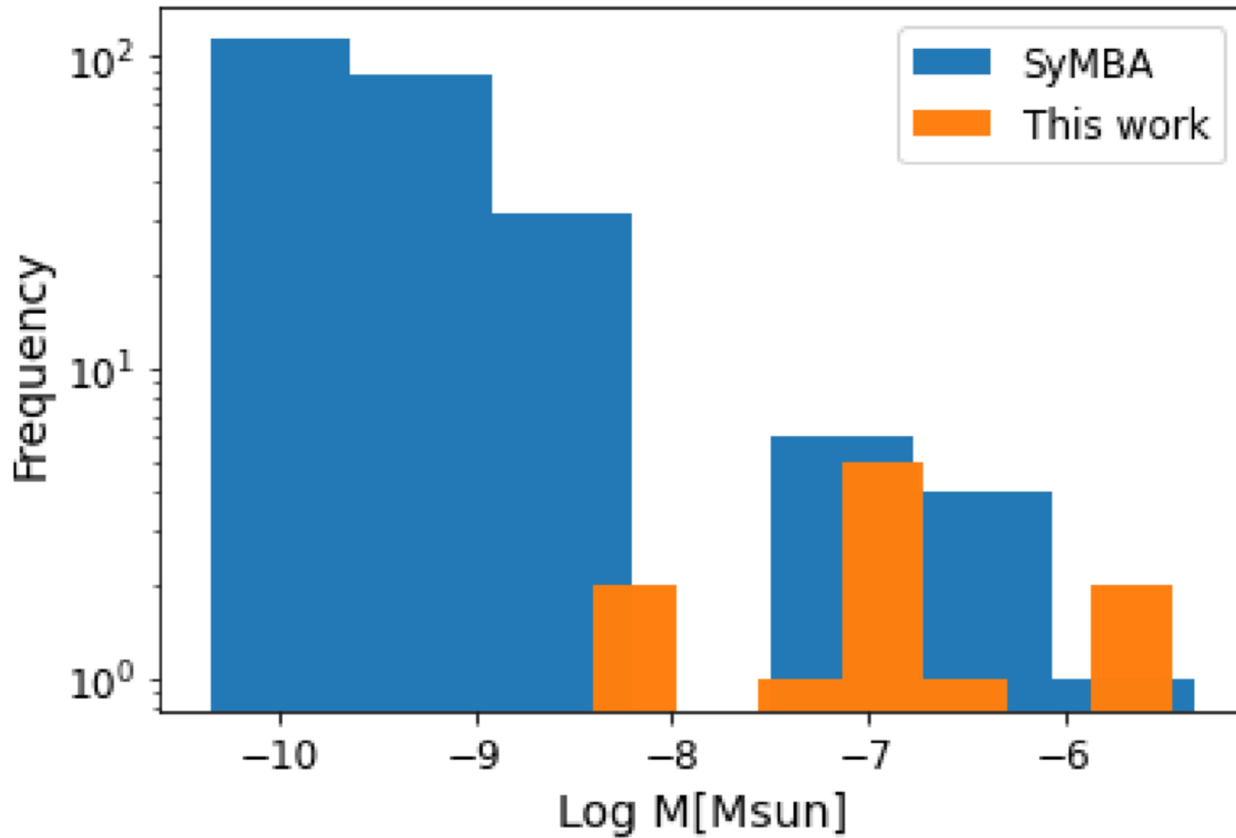
Figure 1. from Samuele Crespi et al 2026 Astron. J. 172 doi:10.3847/1538-3881/ae8ae7 https://dx.doi.org/10.3847/1538-3881/ae8ae7 © 2026. The Author(s). Published by the American Astronomical Society.
