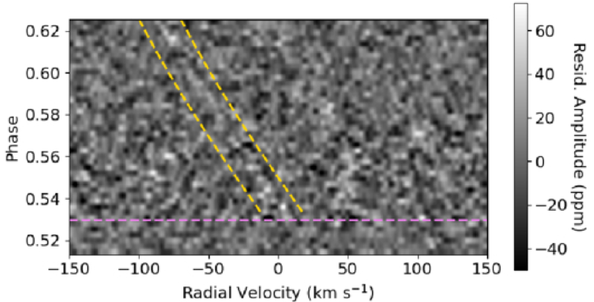
Figure 5. from Aurora Y. Kesseli et al 2026 Astron. J. 172 doi:10.3847/1538-3881/ae8adc https://dx.doi.org/10.3847/1538-3881/ae8adc © 2026. The Author(s). Published by the American Astronomical Society.
