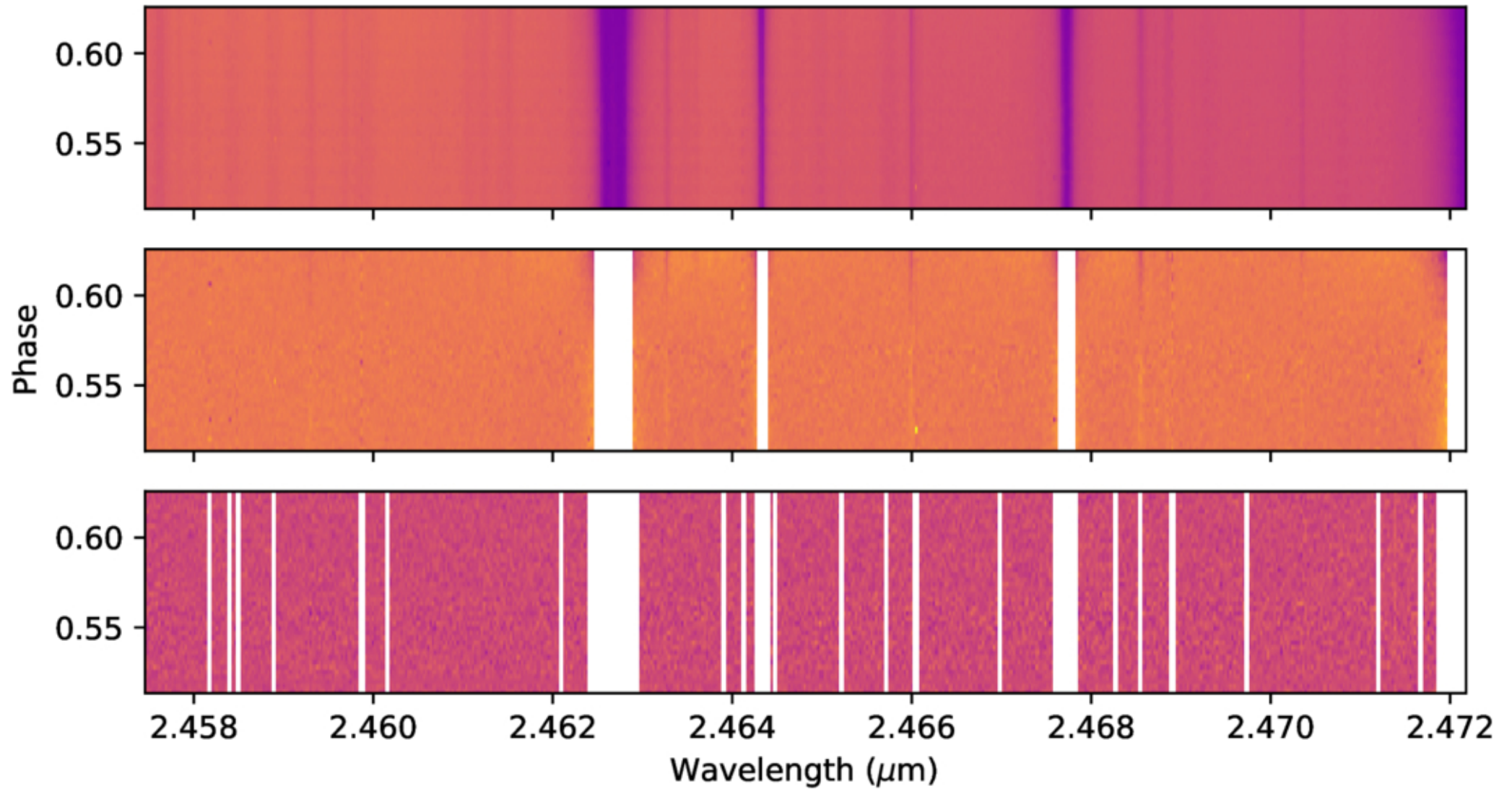
Figure 3. from Aurora Y. Kesseli et al 2026 Astron. J. 172 doi:10.3847/1538-3881/ae8adc https://dx.doi.org/10.3847/1538-3881/ae8adc © 2026. The Author(s). Published by the American Astronomical Society.
