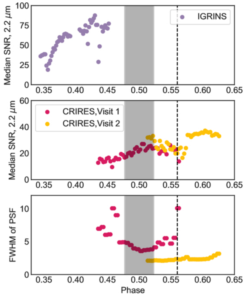
Figure 2. from Aurora Y. Kesseli et al 2026 Astron. J. 172 doi:10.3847/1538-3881/ae8adc https://dx.doi.org/10.3847/1538-3881/ae8adc © 2026. The Author(s). Published by the American Astronomical Society.
