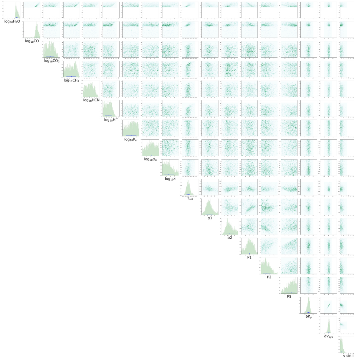
Figure 13. from Aurora Y. Kesseli et al 2026 Astron. J. 172 doi:10.3847/1538-3881/ae8adc https://dx.doi.org/10.3847/1538-3881/ae8adc © 2026. The Author(s). Published by the American Astronomical Society.
