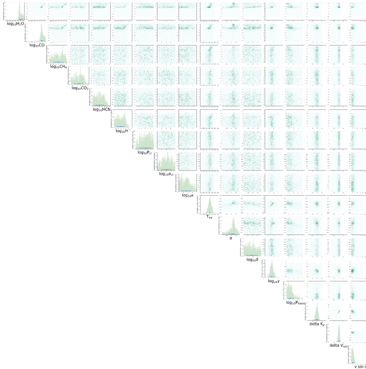
Figure 11. from Aurora Y. Kesseli et al 2026 Astron. J. 172 doi:10.3847/1538-3881/ae8adc https://dx.doi.org/10.3847/1538-3881/ae8adc © 2026. The Author(s). Published by the American Astronomical Society.
