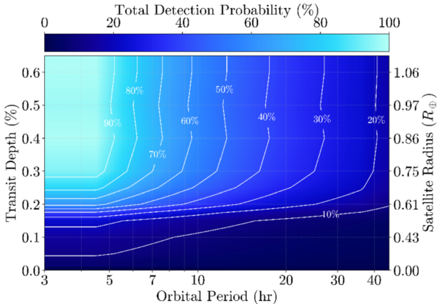
Figure 9. from Brooke Kotten et al 2026 Astron. J. 172 doi:10.3847/1538-3881/ae8adb https://dx.doi.org/10.3847/1538-3881/ae8adb © 2026. The Author(s). Published by the American Astronomical Society.
