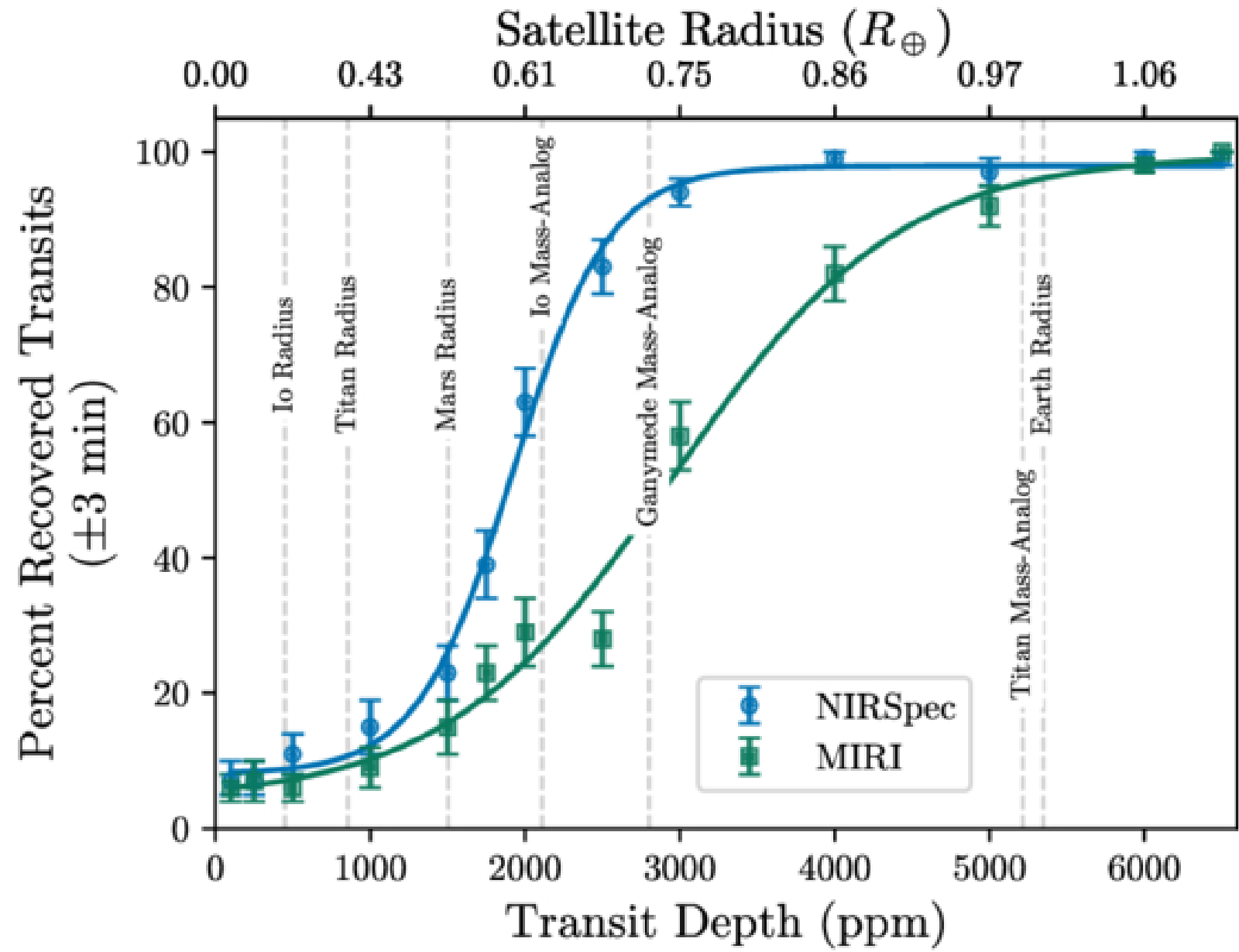
Figure 7. from Brooke Kotten et al 2026 Astron. J. 172 doi:10.3847/1538-3881/ae8adb https://dx.doi.org/10.3847/1538-3881/ae8adb © 2026. The Author(s). Published by the American Astronomical Society.
