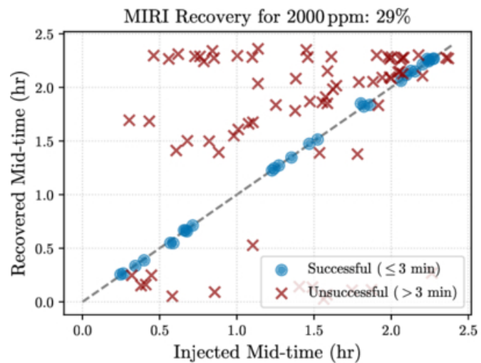
Figure 6. from Brooke Kotten et al 2026 Astron. J. 172 doi:10.3847/1538-3881/ae8adb https://dx.doi.org/10.3847/1538-3881/ae8adb © 2026. The Author(s). Published by the American Astronomical Society.
