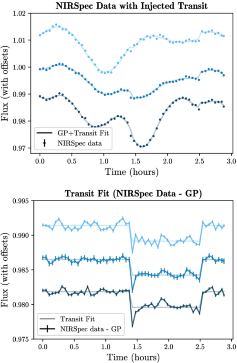
Figure 5. from Brooke Kotten et al 2026 Astron. J. 172 doi:10.3847/1538-3881/ae8adb https://dx.doi.org/10.3847/1538-3881/ae8adb © 2026. The Author(s). Published by the American Astronomical Society.
