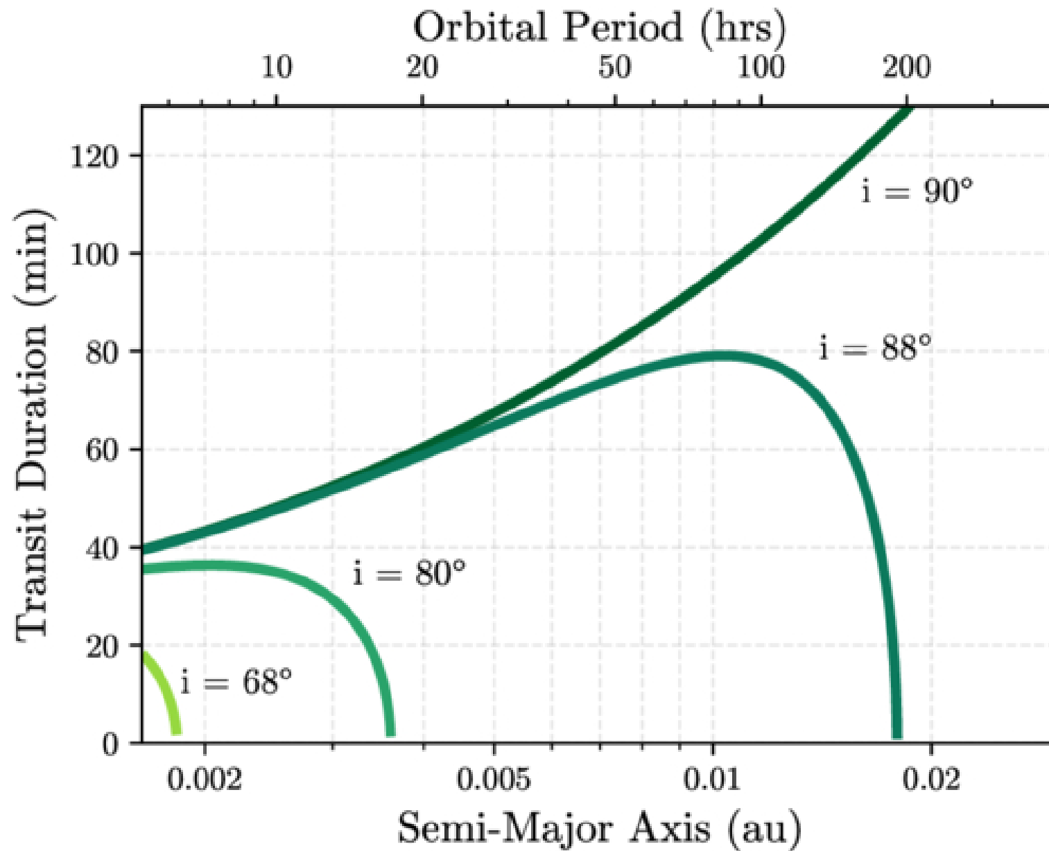
Figure 3. from Brooke Kotten et al 2026 Astron. J. 172 doi:10.3847/1538-3881/ae8adb https://dx.doi.org/10.3847/1538-3881/ae8adb © 2026. The Author(s). Published by the American Astronomical Society.
