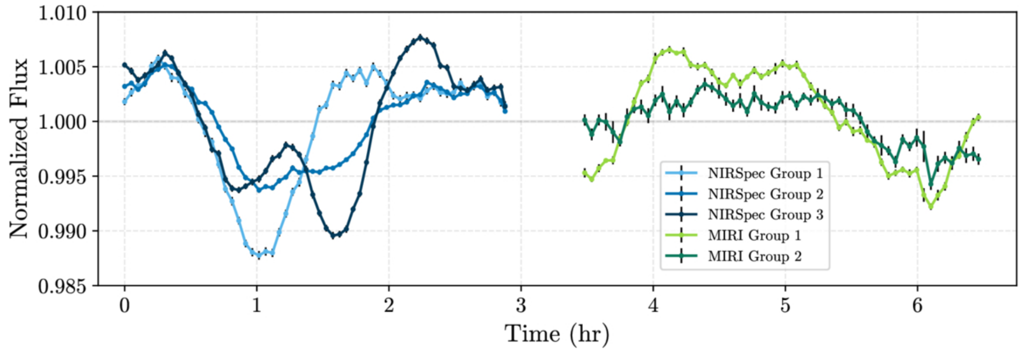
Figure 2. from Brooke Kotten et al 2026 Astron. J. 172 doi:10.3847/1538-3881/ae8adb https://dx.doi.org/10.3847/1538-3881/ae8adb © 2026. The Author(s). Published by the American Astronomical Society.
