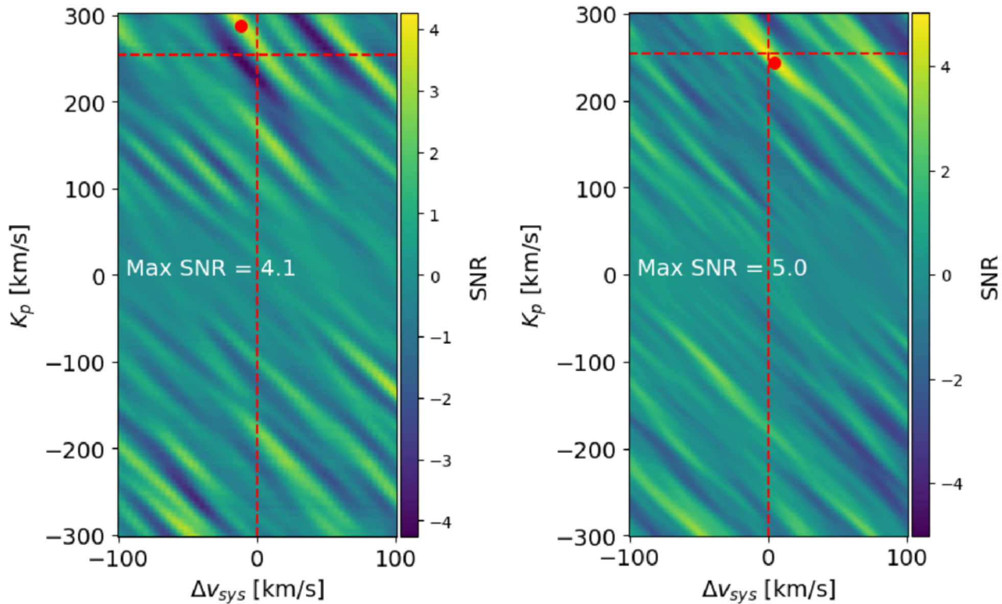
Figure 9. from Luke Finnerty et al 2026 Astron. J. 172 doi:10.3847/1538-3881/ae88f6 https://dx.doi.org/10.3847/1538-3881/ae88f6 © 2026. The Author(s). Published by the American Astronomical Society.
