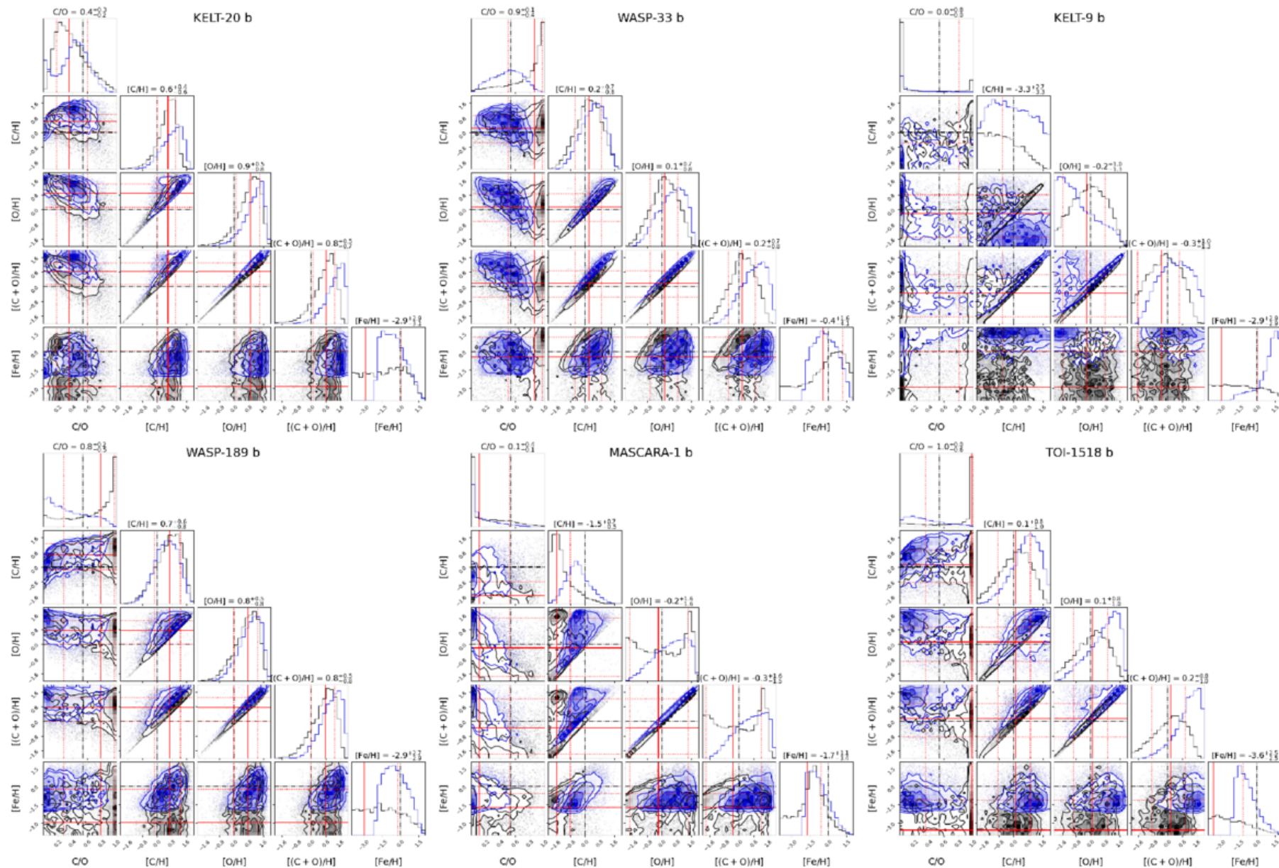
Figure 8. from Luke Finnerty et al 2026 Astron. J. 172 doi:10.3847/1538-3881/ae88f6 https://dx.doi.org/10.3847/1538-3881/ae88f6 © 2026. The Author(s). Published by the American Astronomical Society.
