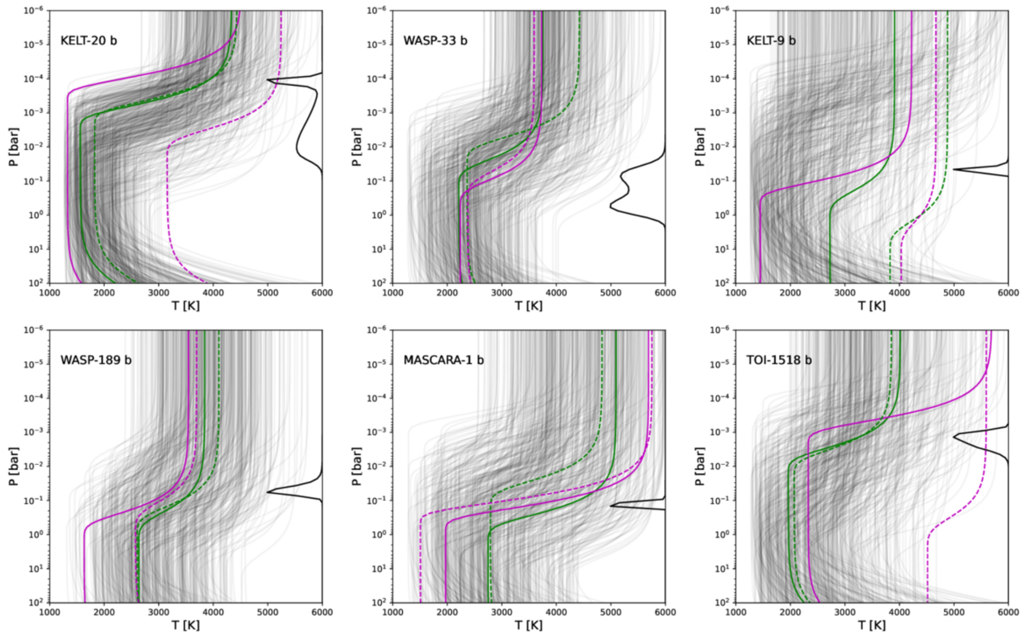
Figure 5. from Luke Finnerty et al 2026 Astron. J. 172 doi:10.3847/1538-3881/ae88f6 https://dx.doi.org/10.3847/1538-3881/ae88f6 © 2026. The Author(s). Published by the American Astronomical Society.
