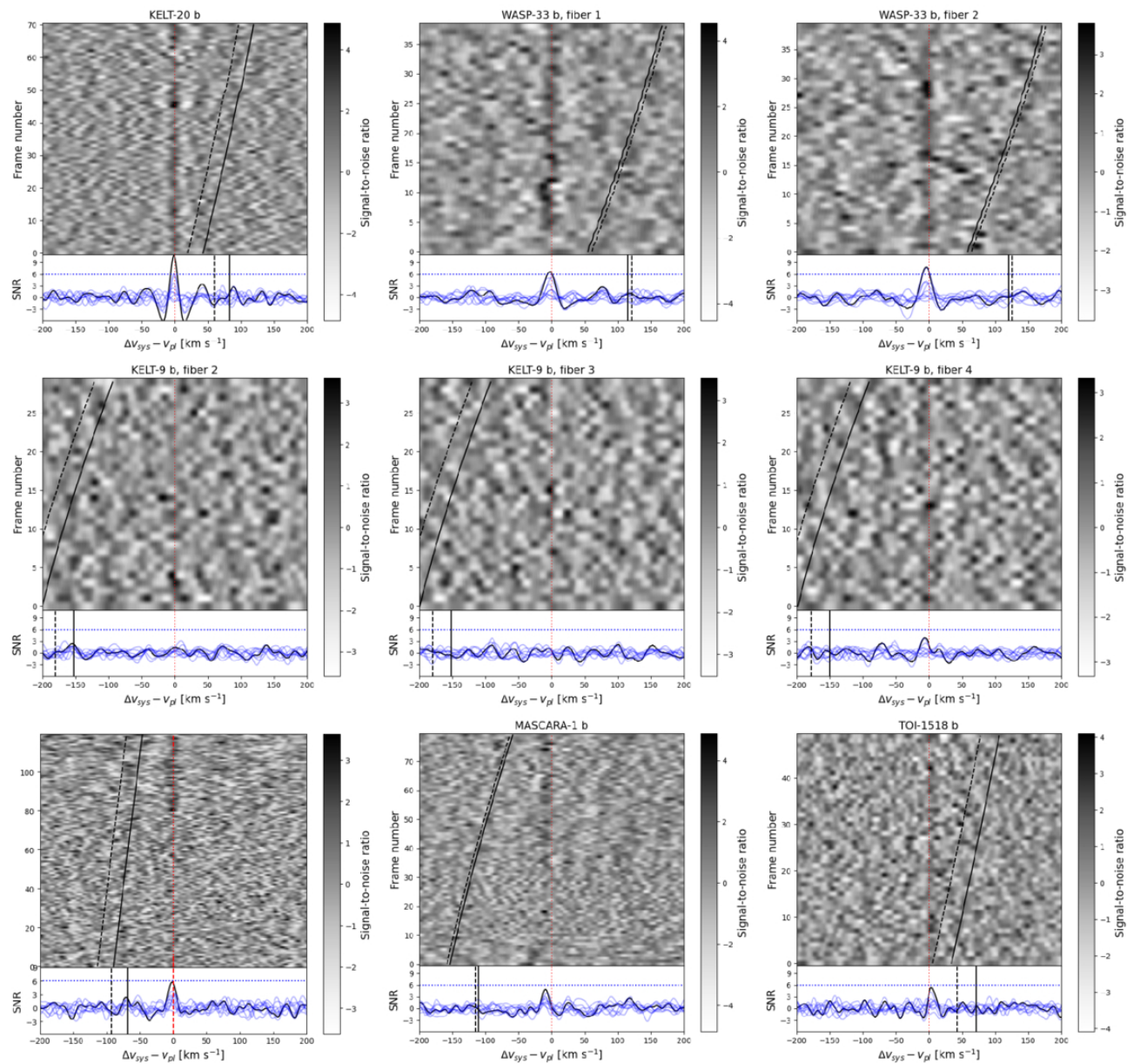
Figure 2. from Luke Finnerty et al 2026 Astron. J. 172 doi:10.3847/1538-3881/ae88f6 https://dx.doi.org/10.3847/1538-3881/ae88f6 © 2026. The Author(s). Published by the American Astronomical Society.
