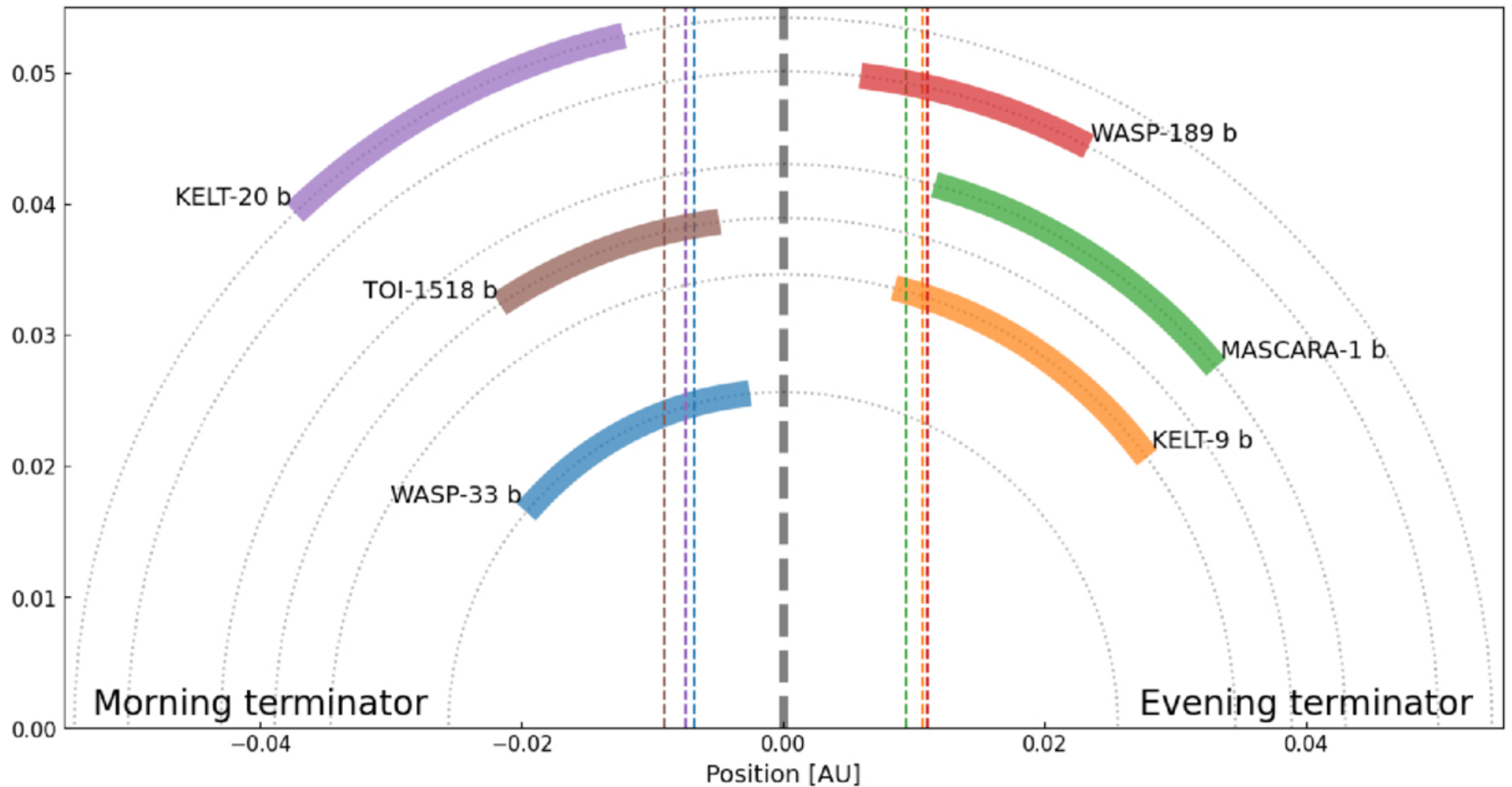
Figure 1. from Luke Finnerty et al 2026 Astron. J. 172 doi:10.3847/1538-3881/ae88f6 https://dx.doi.org/10.3847/1538-3881/ae88f6 © 2026. The Author(s). Published by the American Astronomical Society.
