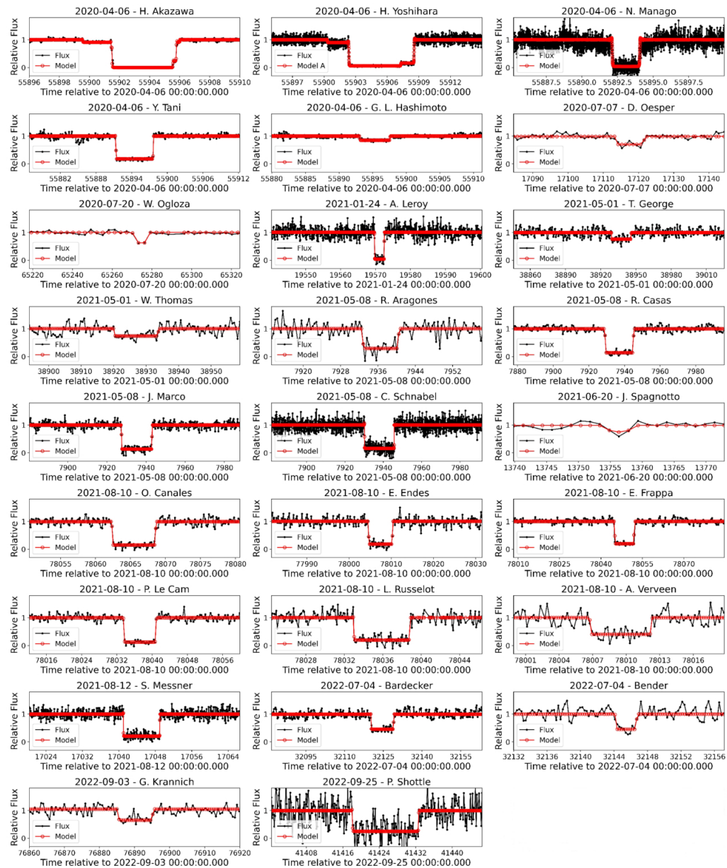
Figure 7. from Luan M. Catani et al 2026 Astron. J. 172 doi:10.3847/1538-3881/ae88f3 https://dx.doi.org/10.3847/1538-3881/ae88f3 © 2026. The Author(s). Published by the American Astronomical Society.
