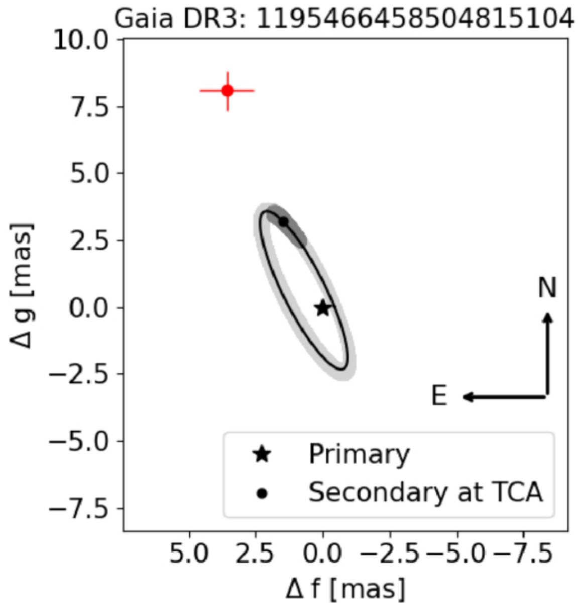
Figure 6. from Luan M. Catani et al 2026 Astron. J. 172 doi:10.3847/1538-3881/ae88f3 https://dx.doi.org/10.3847/1538-3881/ae88f3 © 2026. The Author(s). Published by the American Astronomical Society.
