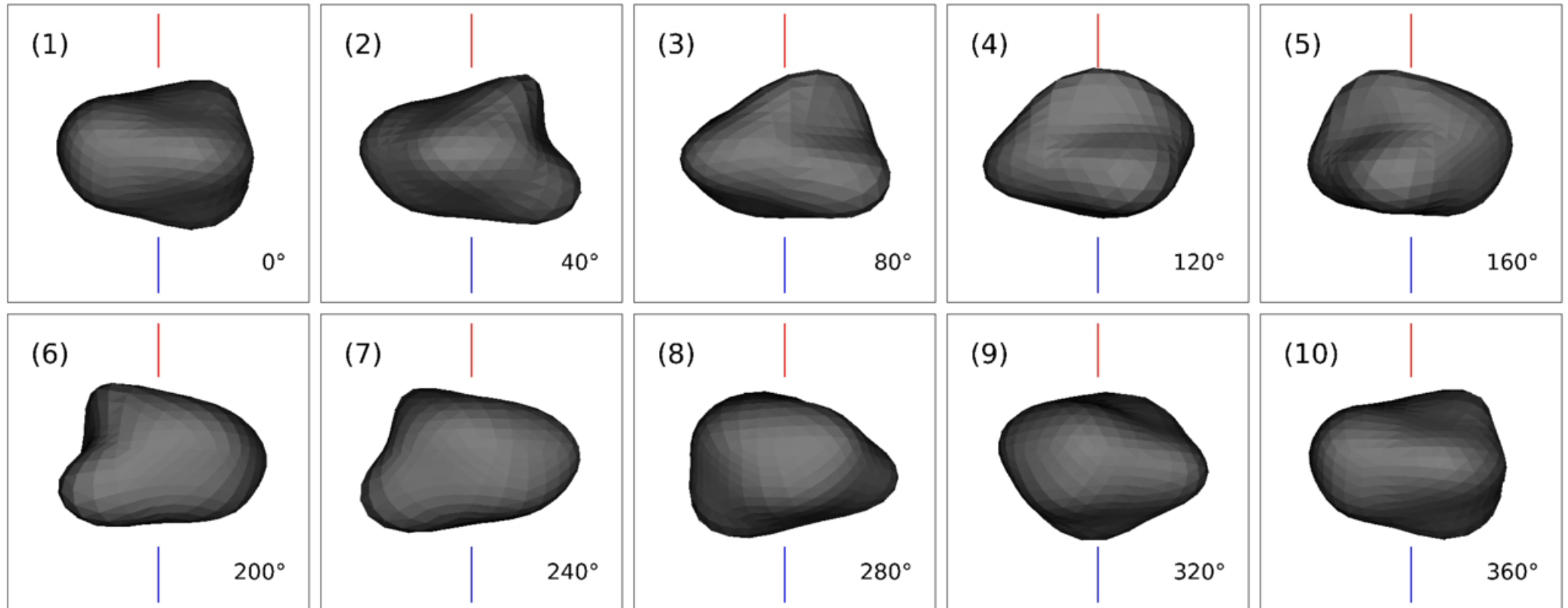
Figure 3. from Luan M. Catani et al 2026 Astron. J. 172 doi:10.3847/1538-3881/ae88f3 https://dx.doi.org/10.3847/1538-3881/ae88f3 © 2026. The Author(s). Published by the American Astronomical Society.
