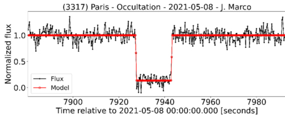
(a) Stellar occultation light curve
