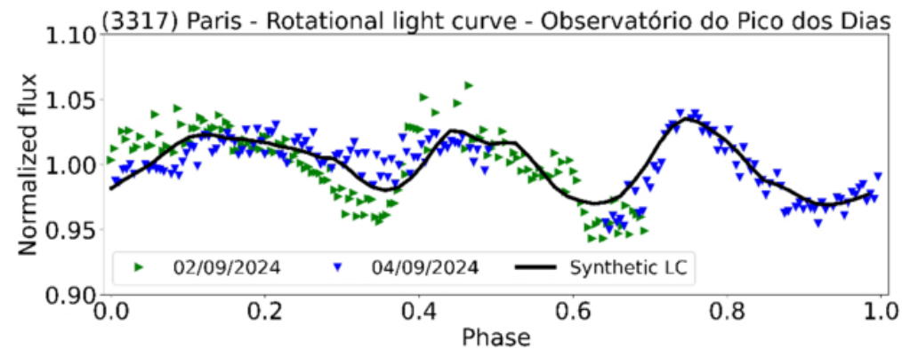
(b) Rotational light curve
