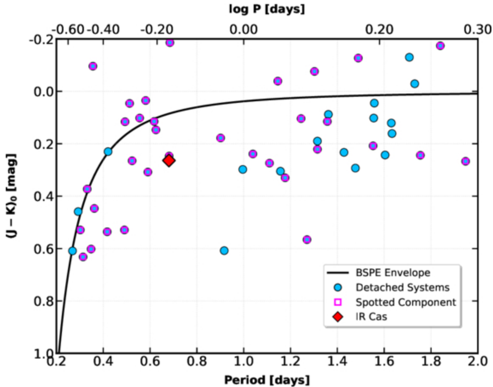
Figure 8. from Matúš Kamenec et al 2026 Astron. J. 172 doi:10.3847/1538-3881/ae87a2 https://dx.doi.org/10.3847/1538-3881/ae87a2 © 2026. The Author(s). Published by the American Astronomical Society.
