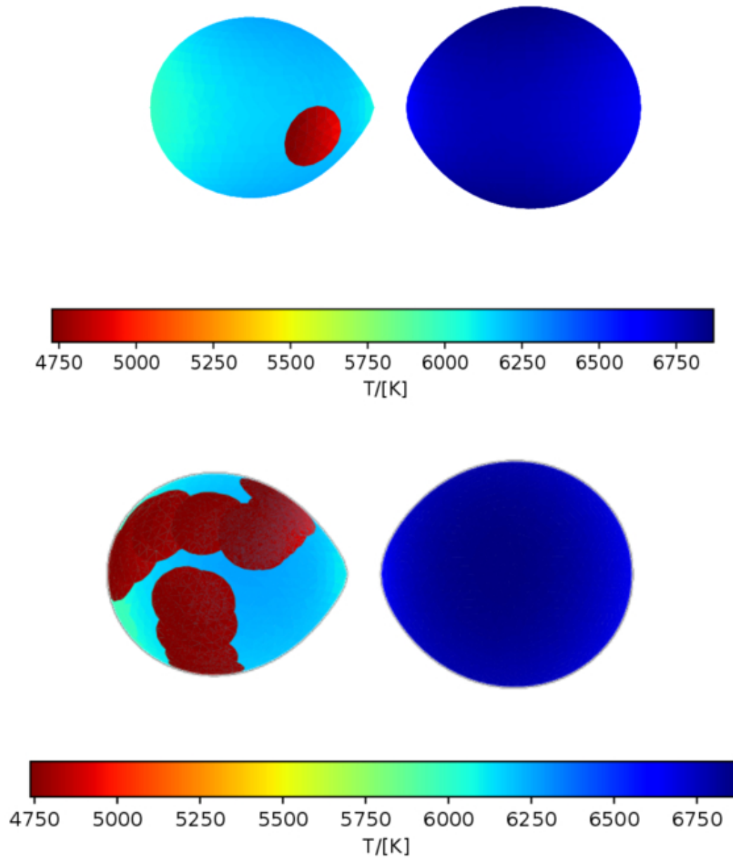
Figure 6. from Matúš Kamenec et al 2026 Astron. J. 172 doi:10.3847/1538-3881/ae87a2 https://dx.doi.org/10.3847/1538-3881/ae87a2 © 2026. The Author(s). Published by the American Astronomical Society.
