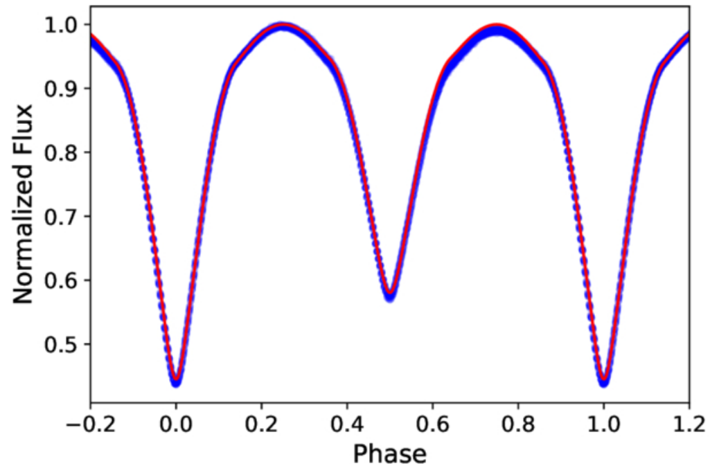
Figure 5. from Matúš Kamenec et al 2026 Astron. J. 172 doi:10.3847/1538-3881/ae87a2 https://dx.doi.org/10.3847/1538-3881/ae87a2 © 2026. The Author(s). Published by the American Astronomical Society.
