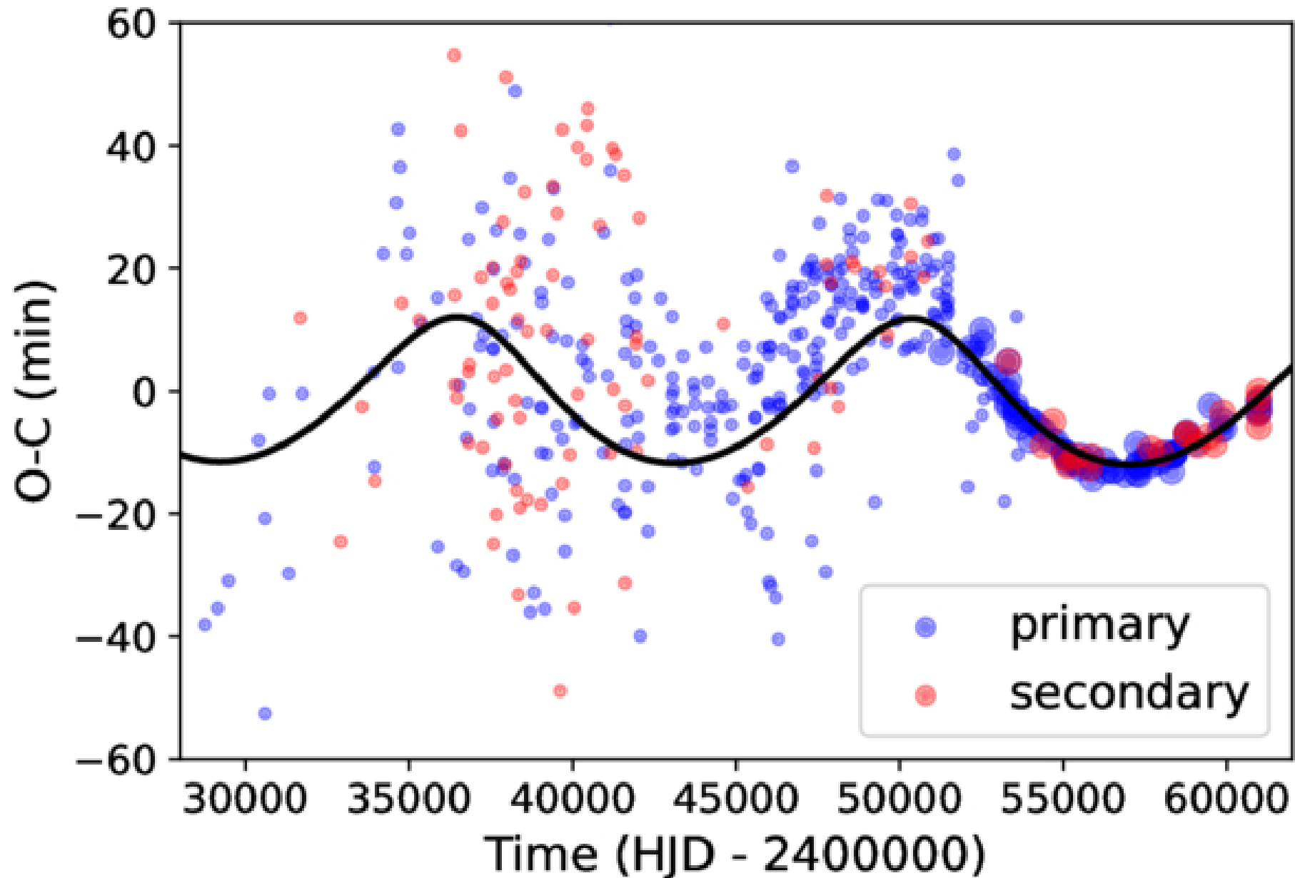
Figure 3. from Matúš Kamenec et al 2026 Astron. J. 172 doi:10.3847/1538-3881/ae87a2 https://dx.doi.org/10.3847/1538-3881/ae87a2 © 2026. The Author(s). Published by the American Astronomical Society.
