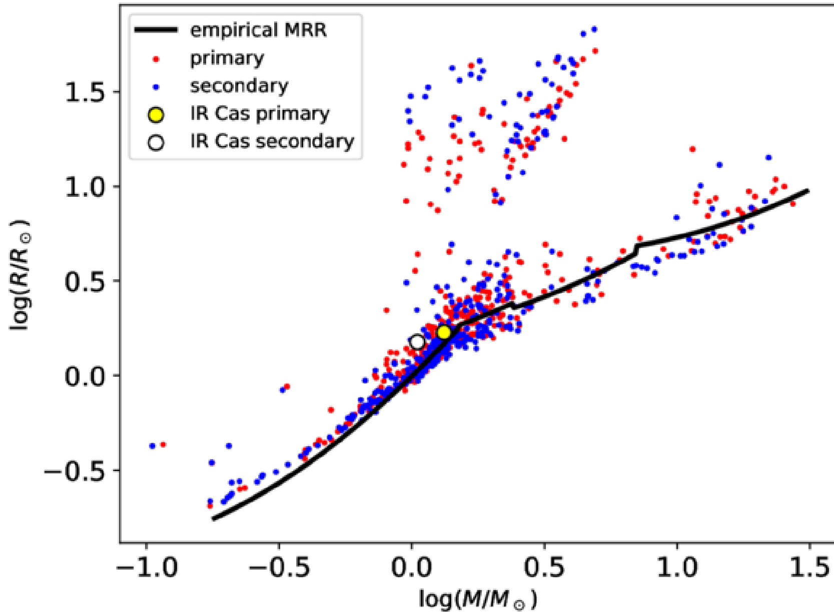
Figure 10. from Matúš Kamenec et al 2026 Astron. J. 172 doi:10.3847/1538-3881/ae87a2 https://dx.doi.org/10.3847/1538-3881/ae87a2 © 2026. The Author(s). Published by the American Astronomical Society.
