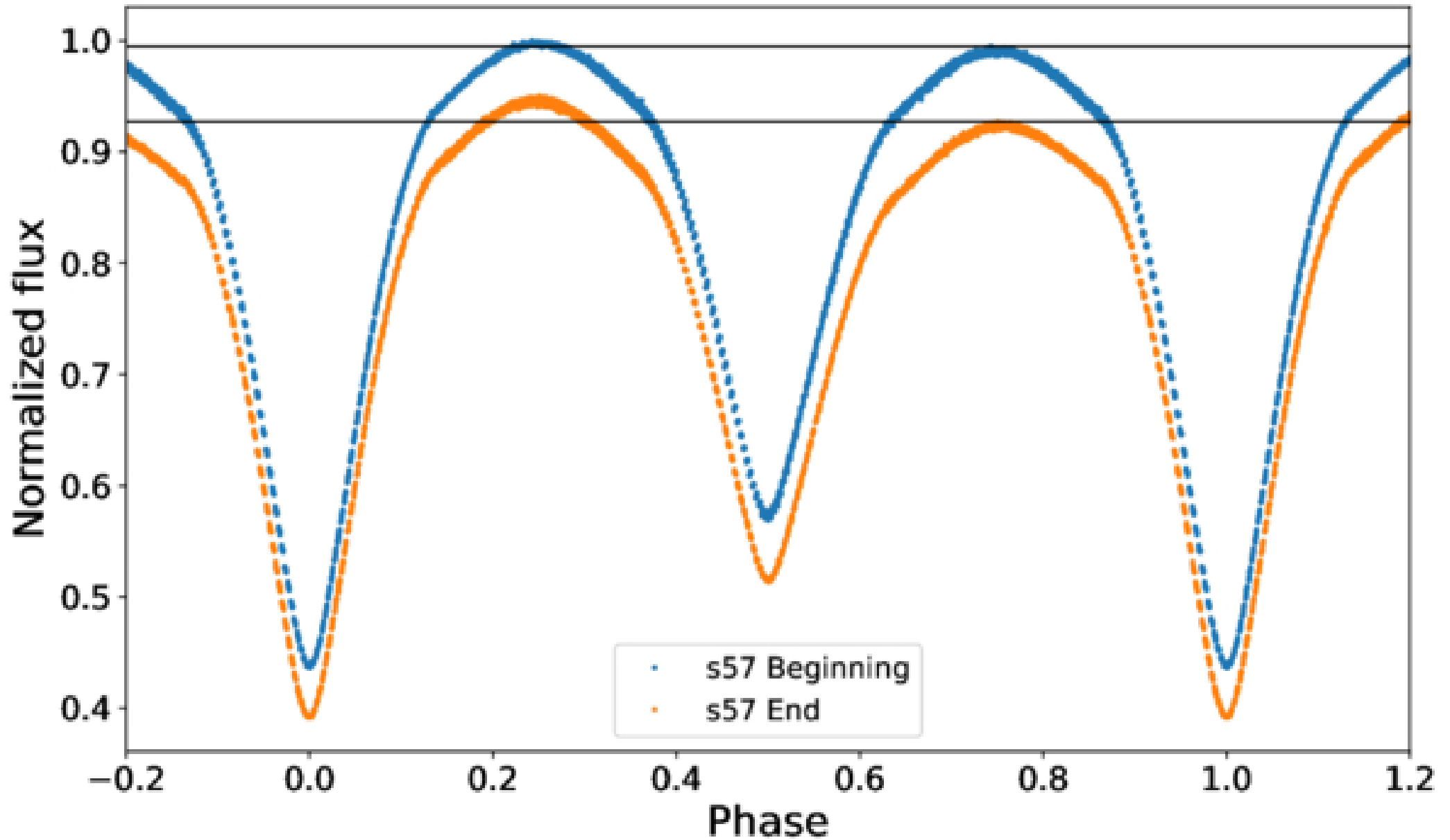
Figure 1. from Matúš Kamenec et al 2026 Astron. J. 172 doi:10.3847/1538-3881/ae87a2 https://dx.doi.org/10.3847/1538-3881/ae87a2 © 2026. The Author(s). Published by the American Astronomical Society.
