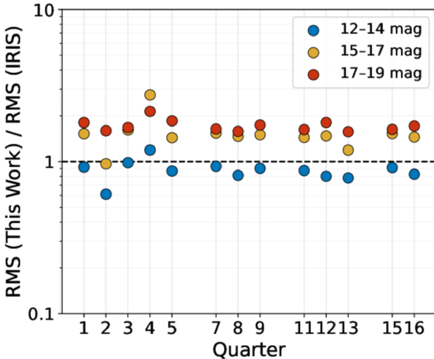
Figure 3. from Melinda Soares-Furtado et al 2026 Astron. J. 172 doi:10.3847/1538-3881/ae877e https://dx.doi.org/10.3847/1538-3881/ae877e © 2026. The Author(s). Published by the American Astronomical Society.
