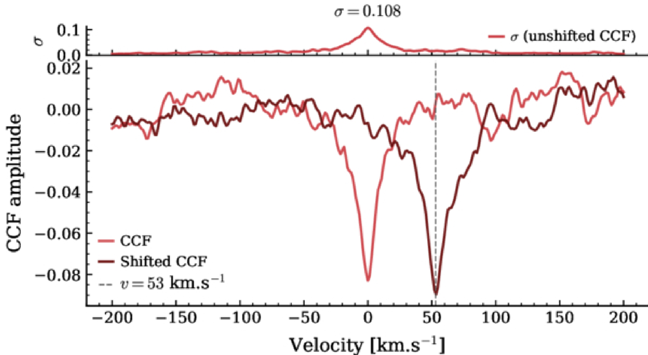
Figure A1. from Evann Kurzawa-Ferrandez et al 2026 Astron. J. 172 doi:10.3847/1538-3881/ae8770 https://dx.doi.org/10.3847/1538-3881/ae8770 © 2026. The Author(s). Published by the American Astronomical Society.
