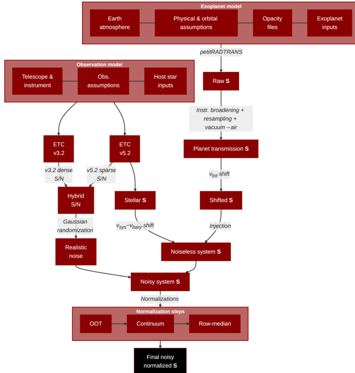
Figure 4. from Evann Kurzawa-Ferrandez et al 2026 Astron. J. 172 doi:10.3847/1538-3881/ae8770 https://dx.doi.org/10.3847/1538-3881/ae8770 © 2026. The Author(s). Published by the American Astronomical Society.
