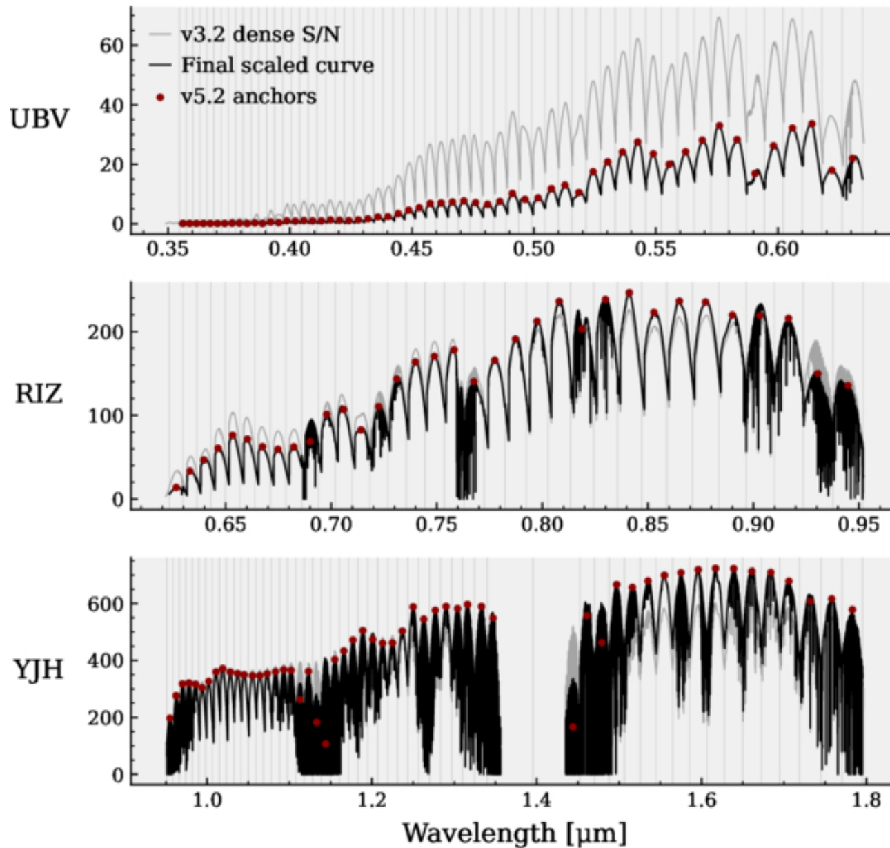
Figure 3. from Evann Kurzawa-Ferrandez et al 2026 Astron. J. 172 doi:10.3847/1538-3881/ae8770 https://dx.doi.org/10.3847/1538-3881/ae8770 © 2026. The Author(s). Published by the American Astronomical Society.
