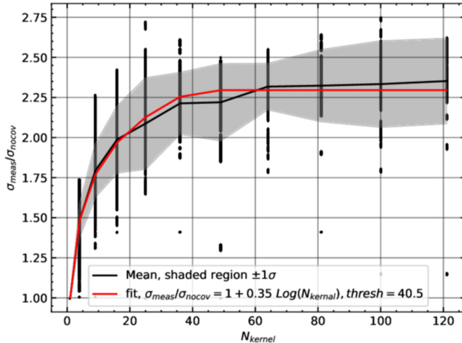
Figure 9. from Zeren Lin and D. Christopher Martin 2026 Astron. J. 172 doi:10.3847/1538-3881/ae84bd https://dx.doi.org/10.3847/1538-3881/ae84bd © 2026. The Author(s). Published by the American Astronomical Society.
