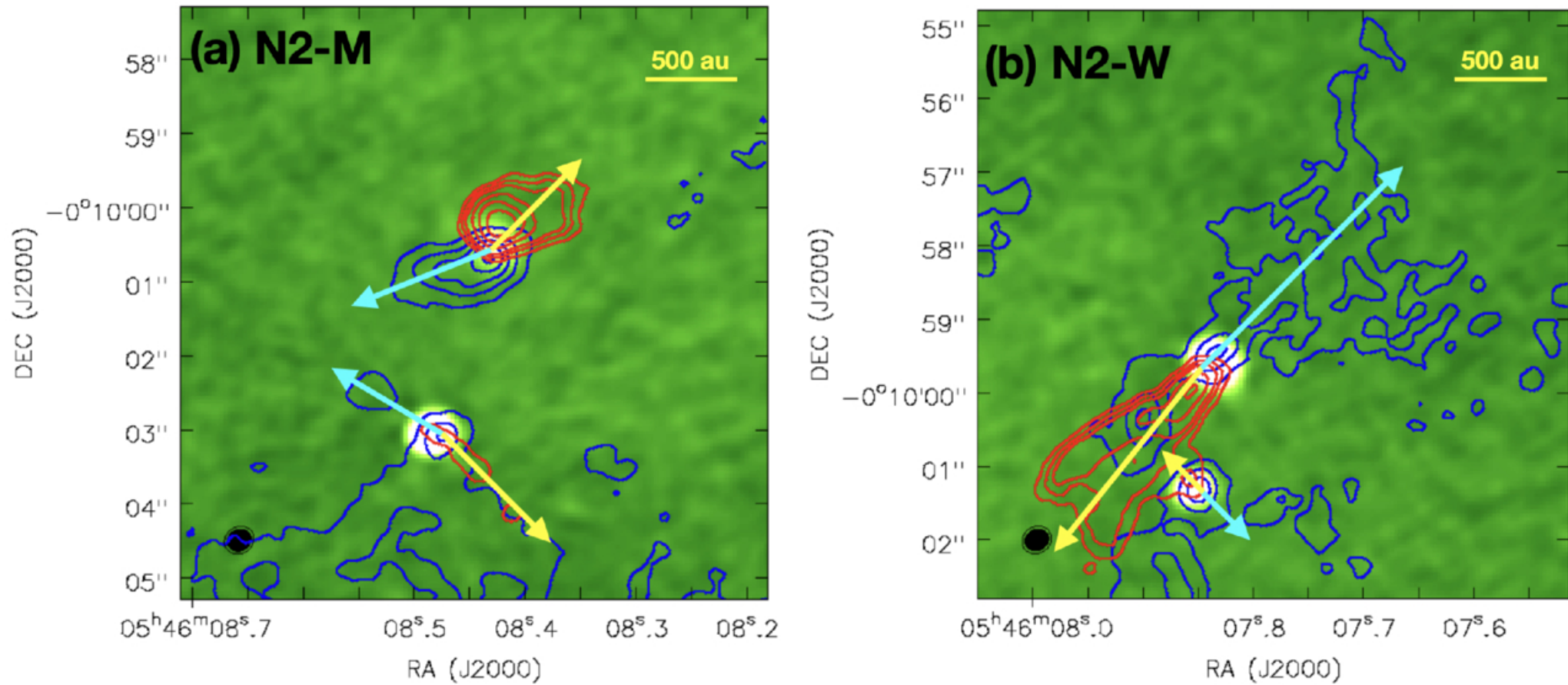
Figure 2. from Tie Liu et al 2026 Astron. J. 172 doi:10.3847/1538-3881/ae83b8 https://dx.doi.org/10.3847/1538-3881/ae83b8 © 2026. The Author(s). Published by the American Astronomical Society.
