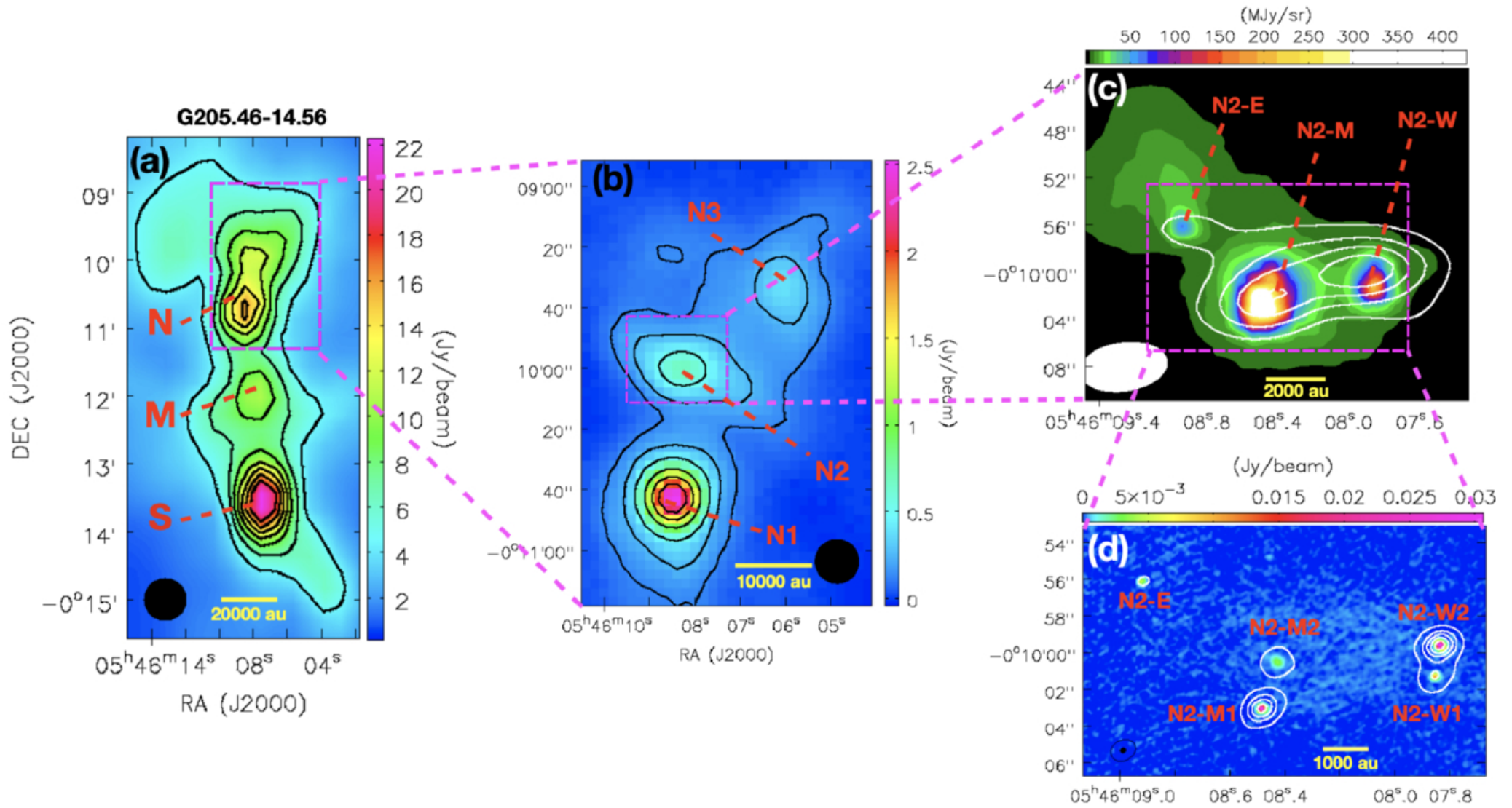
Figure 1. from Tie Liu et al 2026 Astron. J. 172 doi:10.3847/1538-3881/ae83b8 https://dx.doi.org/10.3847/1538-3881/ae83b8 © 2026. The Author(s). Published by the American Astronomical Society.
