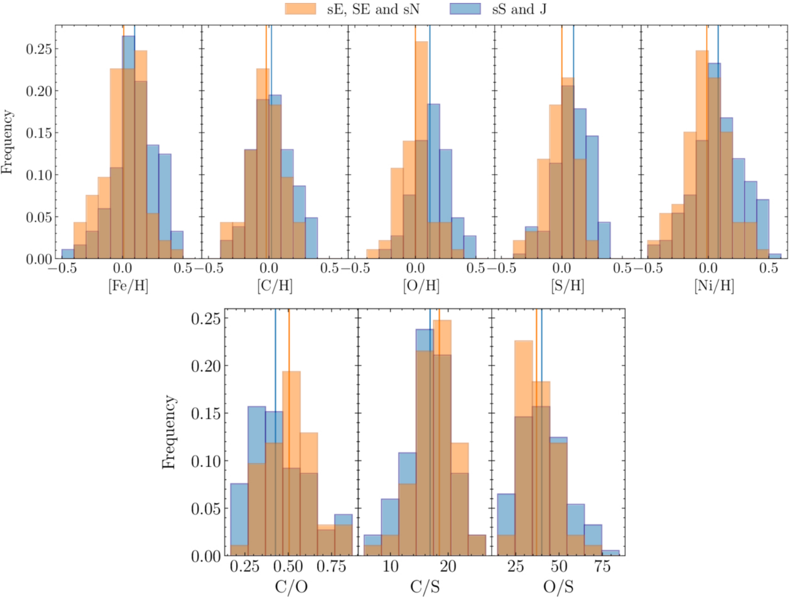
Figure 8. from Ellen Costa-Almeida et al 2026 Astron. J. 172 doi:10.3847/1538-3881/ae82fd https://dx.doi.org/10.3847/1538-3881/ae82fd © 2026. The Author(s). Published by the American Astronomical Society.
