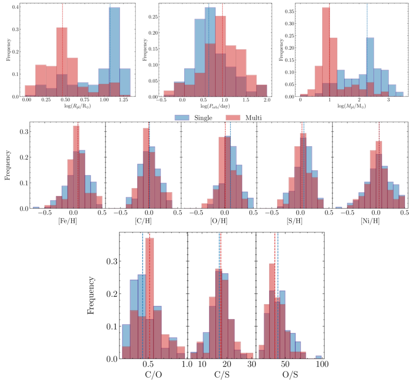
Figure 7. from Ellen Costa-Almeida et al 2026 Astron. J. 172 doi:10.3847/1538-3881/ae82fd https://dx.doi.org/10.3847/1538-3881/ae82fd © 2026. The Author(s). Published by the American Astronomical Society.
