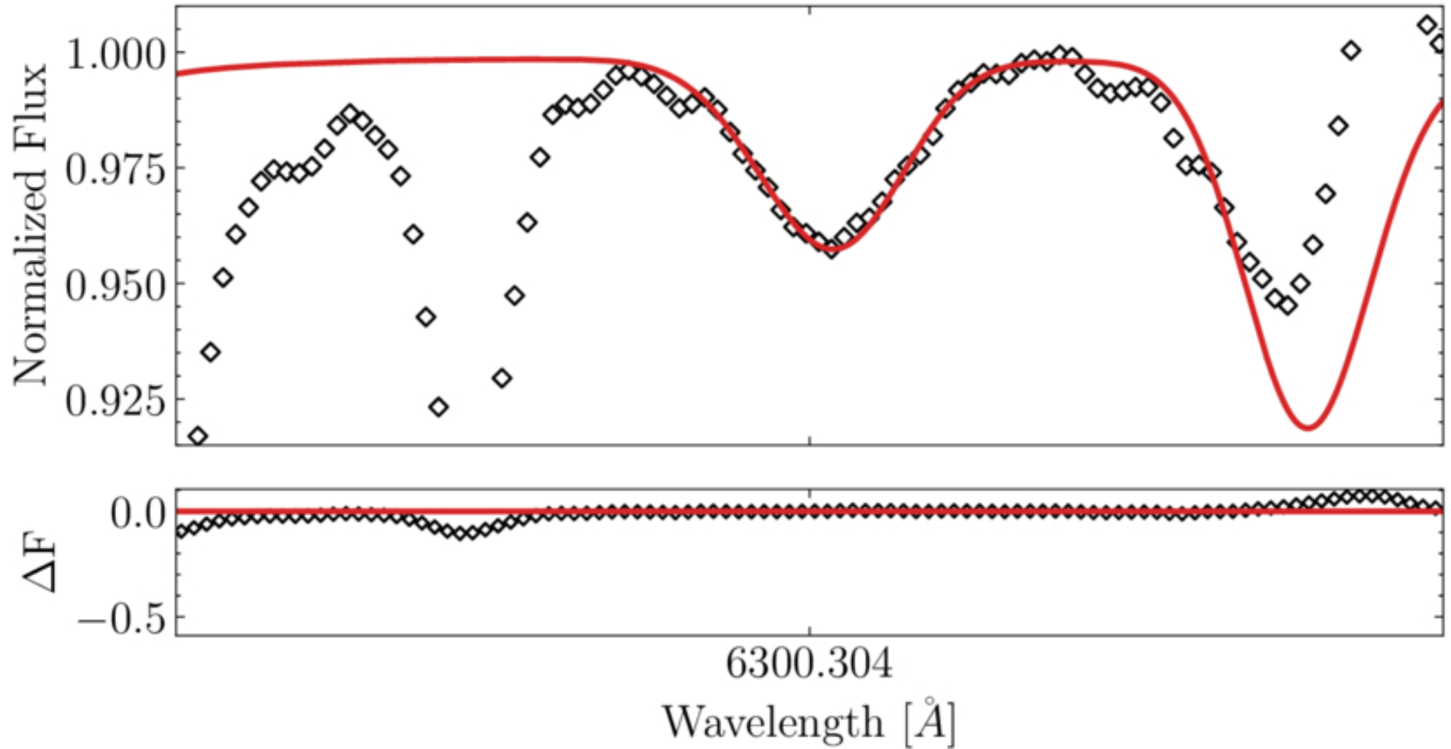
Figure 4. from Ellen Costa-Almeida et al 2026 Astron. J. 172 doi:10.3847/1538-3881/ae82fd https://dx.doi.org/10.3847/1538-3881/ae82fd © 2026. The Author(s). Published by the American Astronomical Society.
