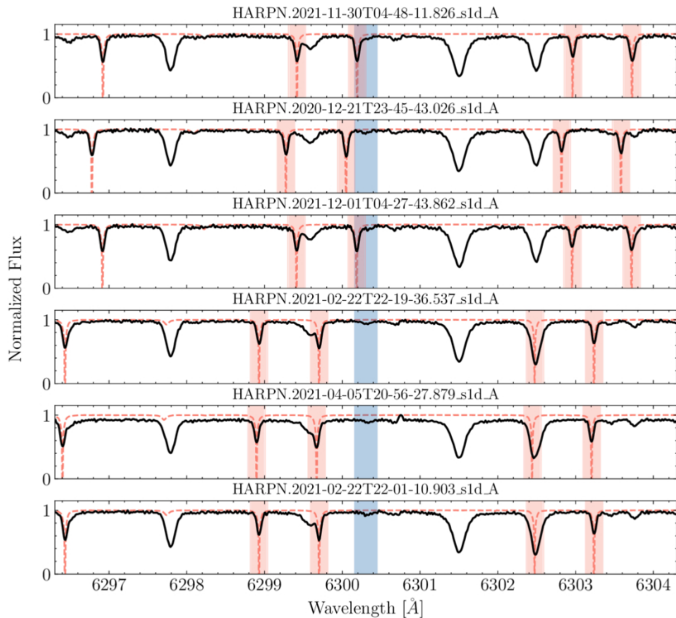
Figure 3. from Ellen Costa-Almeida et al 2026 Astron. J. 172 doi:10.3847/1538-3881/ae82fd https://dx.doi.org/10.3847/1538-3881/ae82fd © 2026. The Author(s). Published by the American Astronomical Society.
