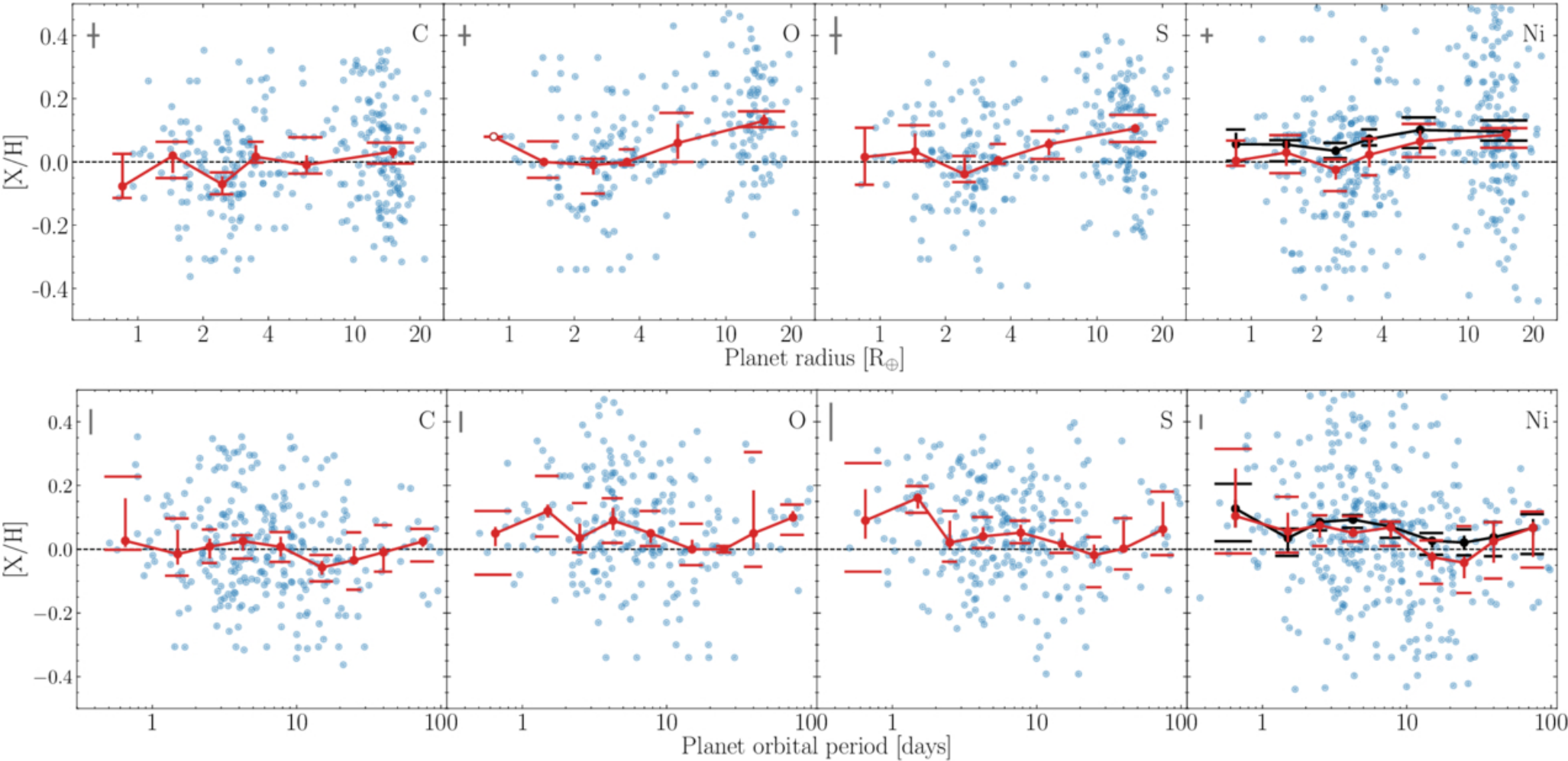
Figure 10. from Ellen Costa-Almeida et al 2026 Astron. J. 172 doi:10.3847/1538-3881/ae82fd https://dx.doi.org/10.3847/1538-3881/ae82fd © 2026. The Author(s). Published by the American Astronomical Society.
