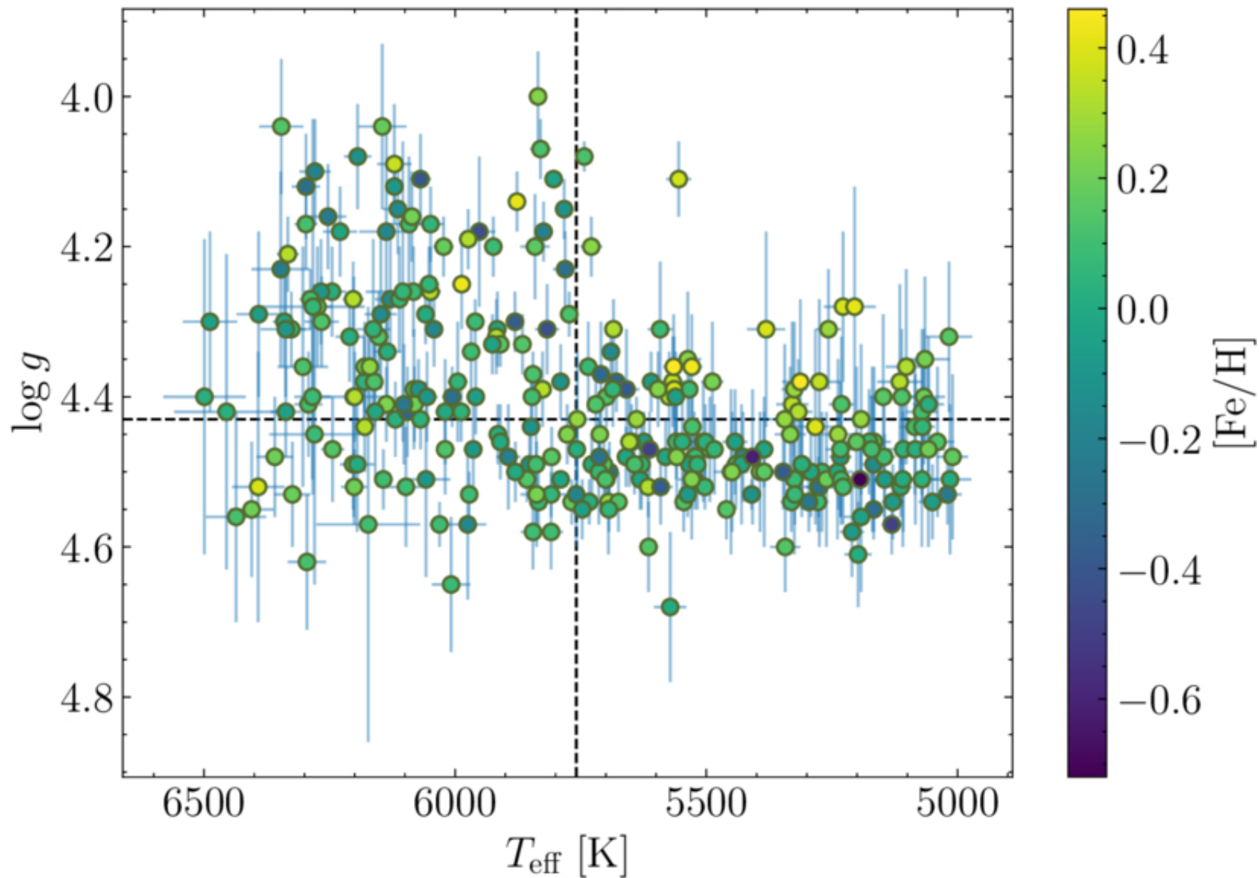
Figure 1. from Ellen Costa-Almeida et al 2026 Astron. J. 172 doi:10.3847/1538-3881/ae82fd https://dx.doi.org/10.3847/1538-3881/ae82fd © 2026. The Author(s). Published by the American Astronomical Society.
