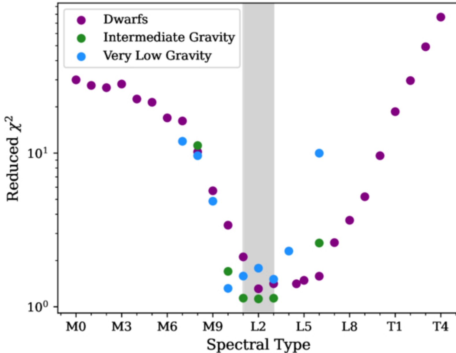
Figure 7. from Marah Brinjikji et al 2026 Astron. J. 172 doi:10.3847/1538-3881/ae82f2 https://dx.doi.org/10.3847/1538-3881/ae82f2 © 2026. The Author(s). Published by the American Astronomical Society.
