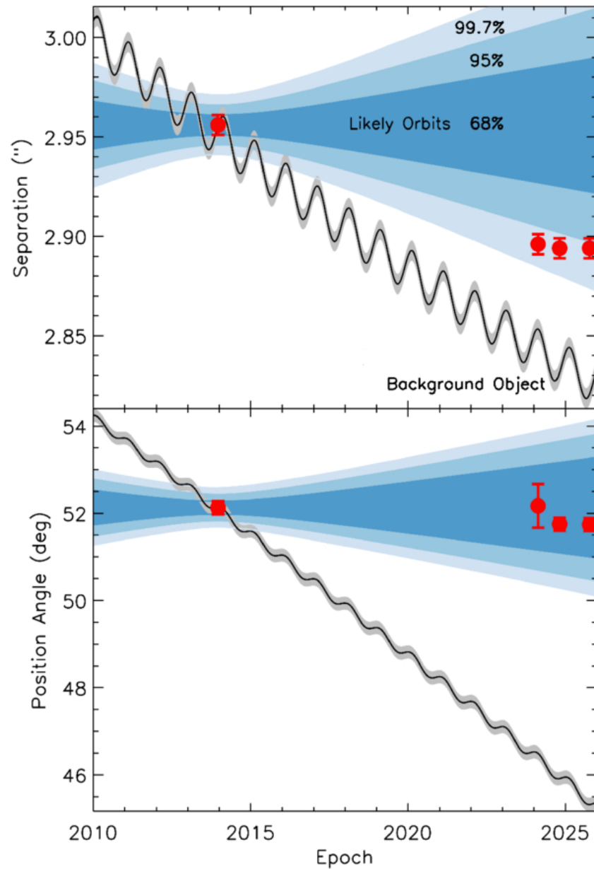
Figure 3. from Marah Brinjikji et al 2026 Astron. J. 172 doi:10.3847/1538-3881/ae82f2 https://dx.doi.org/10.3847/1538-3881/ae82f2 © 2026. The Author(s). Published by the American Astronomical Society.
