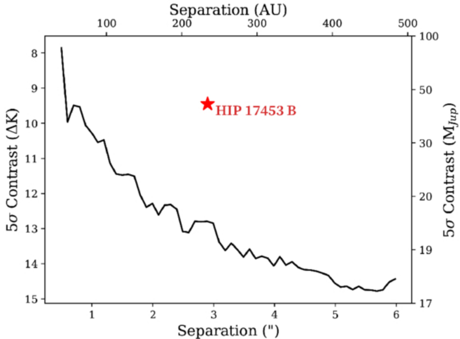
Figure 2. from Marah Brinjikji et al 2026 Astron. J. 172 doi:10.3847/1538-3881/ae82f2 https://dx.doi.org/10.3847/1538-3881/ae82f2 © 2026. The Author(s). Published by the American Astronomical Society.
