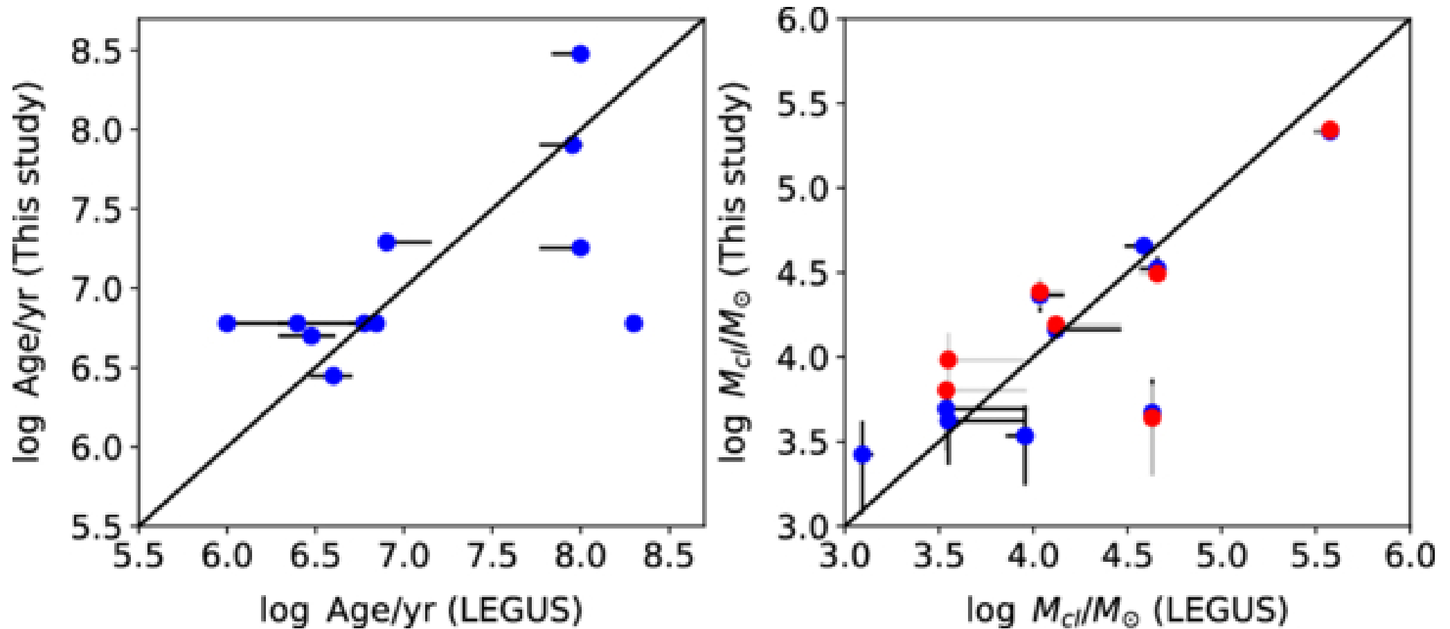
Figure 8. from Jae-Rim Koo et al 2026 Astron. J. 172 doi:10.3847/1538-3881/ae8250 https://dx.doi.org/10.3847/1538-3881/ae8250 © 2026. The Author(s). Published by the American Astronomical Society.
