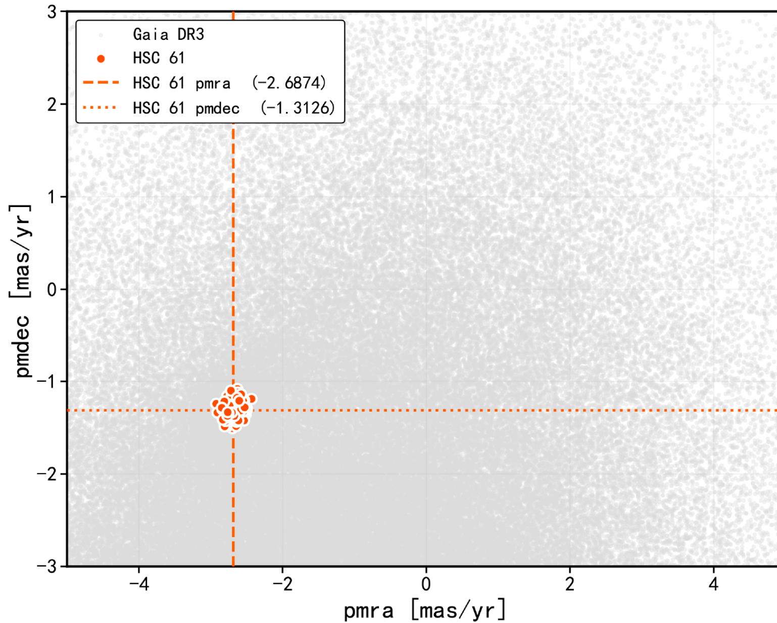
Figure 8. from P. Wang et al 2026 Astron. J. 172 doi:10.3847/1538-3881/ae81b5 https://dx.doi.org/10.3847/1538-3881/ae81b5 © 2026. The Author(s). Published by the American Astronomical Society.
